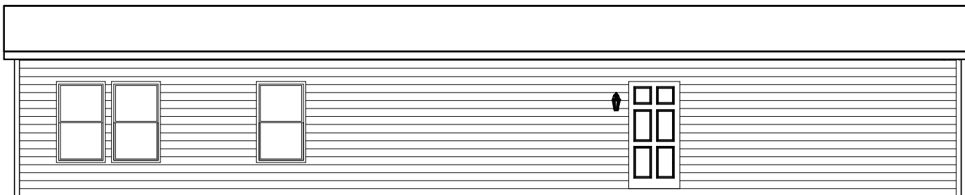
BACK ELEVATION
