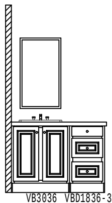
CABINET ELEVATION E STANDARD BATH
