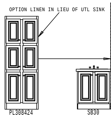
CABINET ELEVATION F OPTION UTILITY SINK
